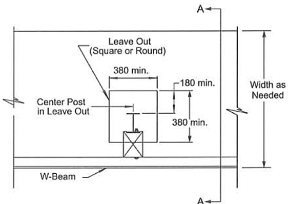
Steel Post Detail (Metric)
