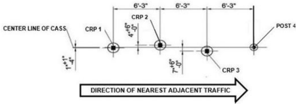
Figure 1a CRP Offset 3 Cable system
