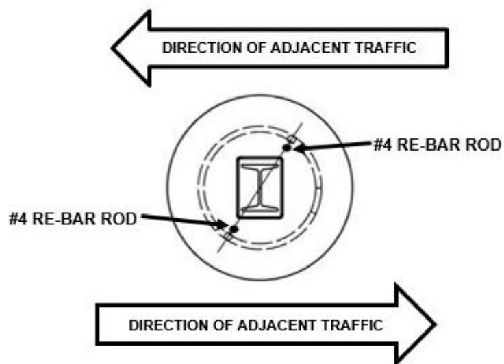
Figure 3 CCT Re-bar Placement
