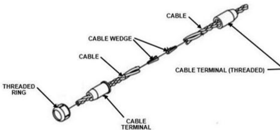
Figure 7 Torpedo Cable Splice
