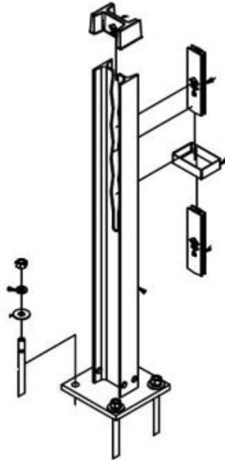
Figure 15 Base Plated Post
