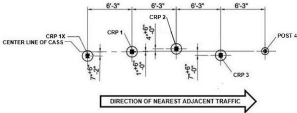
Figure 1b CRP Offset 4 Cable system
