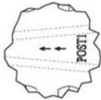
DETAIL E ORIENTATION OF SRT™ SLOT GUARD POINTING TOWARD POST 1
