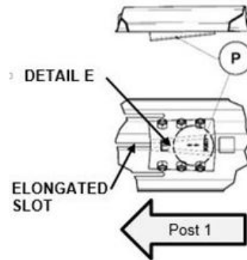
SRT™ SLOT GUARD DETAIL NON-TRAFFIC SIDE
