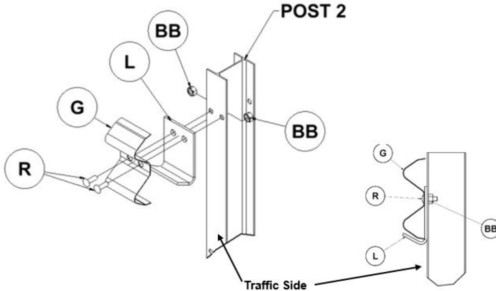
COMPLETED ASSEMBLY DETAIL
