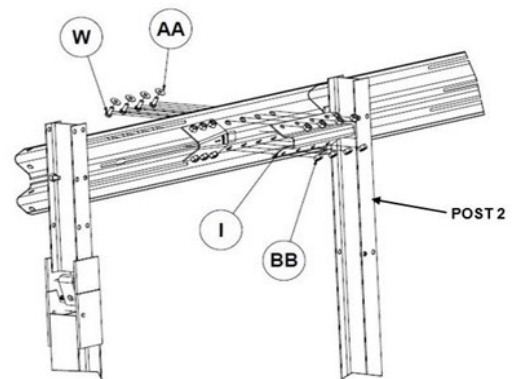
VIEW FROM NONTRAFFIC SIDE
