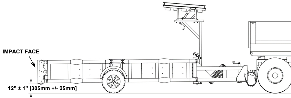
Figure 12 Trailer Attachment to Support Truck
